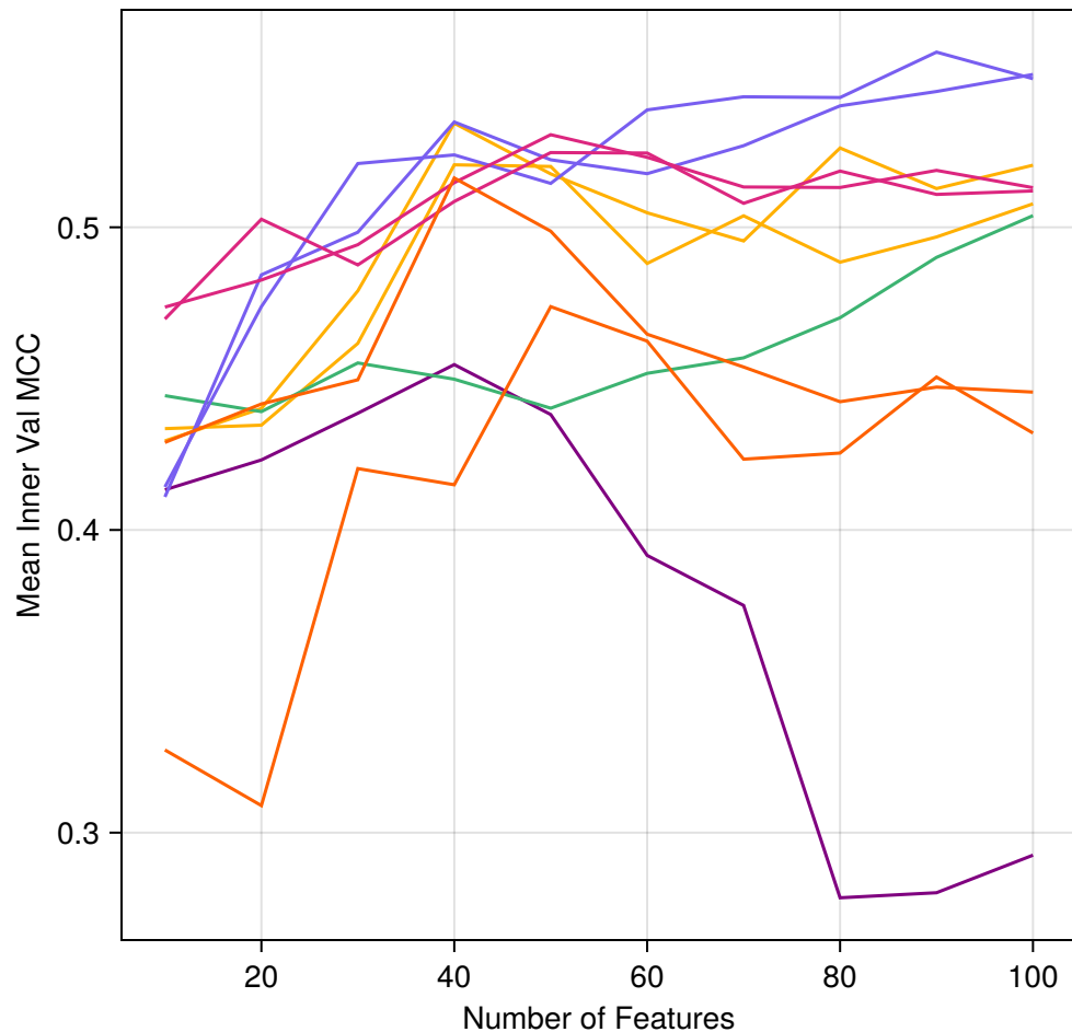
sex aware — Boruta
